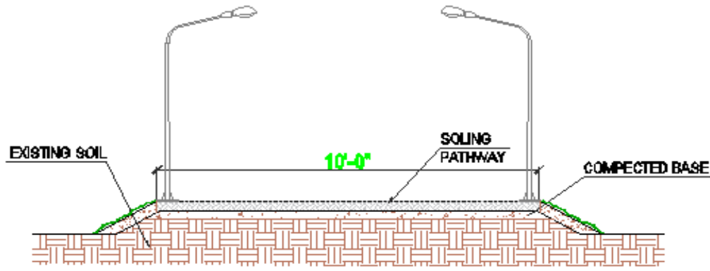
PATHWAY CROSS SECTION
