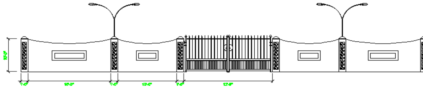
BOUNDARY WALL / GATE
