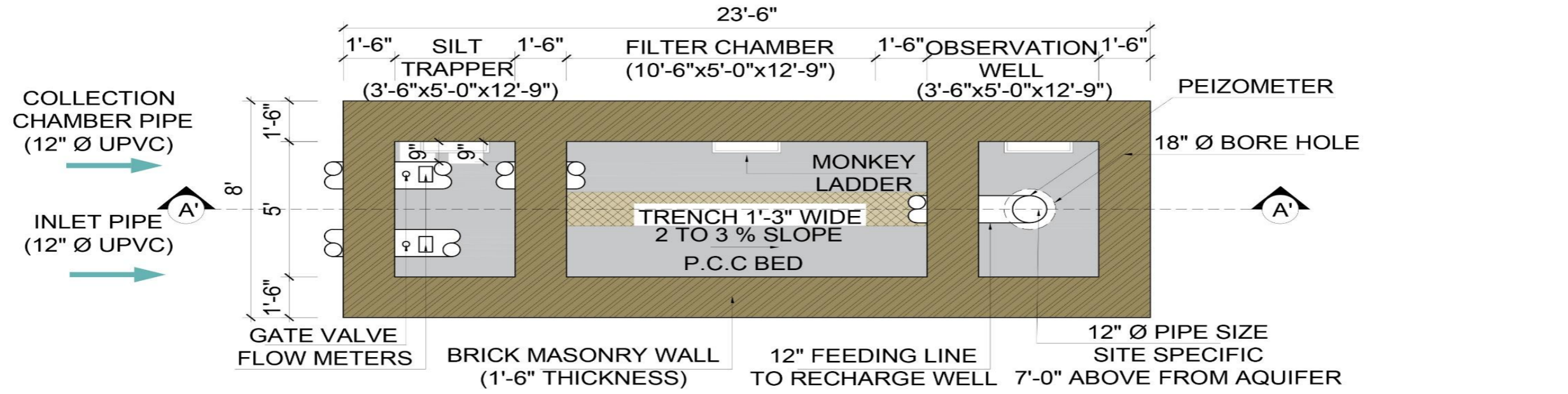
TOP VIEW (UNCOVERED) PLAN SITE COVERED AREA (188 Sq.ft)
